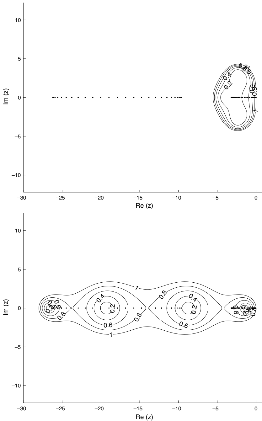
Fig. 4. The stability domain S and values -\lambda\mu_i (dots) for the EXI method (top) and EXV method (bottom) in the time-dependent viscous flow regime with \lambda = 8 \times 10^{-3} . The pseudo-time Von Neumann number is 0.8 and for this constraint only the EXV method is stable.
