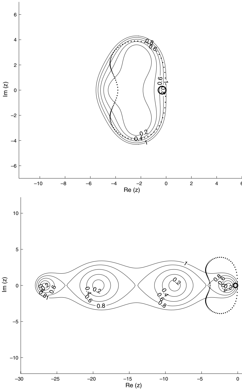
Fig. 1. The stability domain S and values -\lambda\mu_i (dots) for the EXI method (top) and EXV method (bottom) in the steady-state inviscid flow regime with \lambda = 1.8 \times 10^{-2} . The pseudo-time CFL number is 1.8 and for this constraint only the EXI method is stable.
